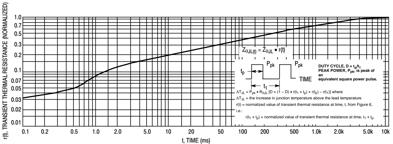
Figure 6. Thermal Response
