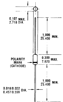
FIGURE 1 All dimensions in \frac{\text{INCH}}{\text{m.m.}}
