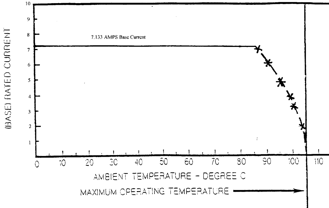
Figure 4A Current Carrying Capability
