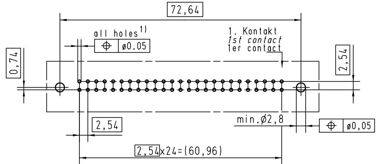
Printed Board Layout Component side
