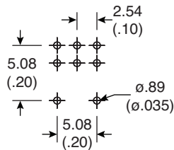
P.C. Mounting
